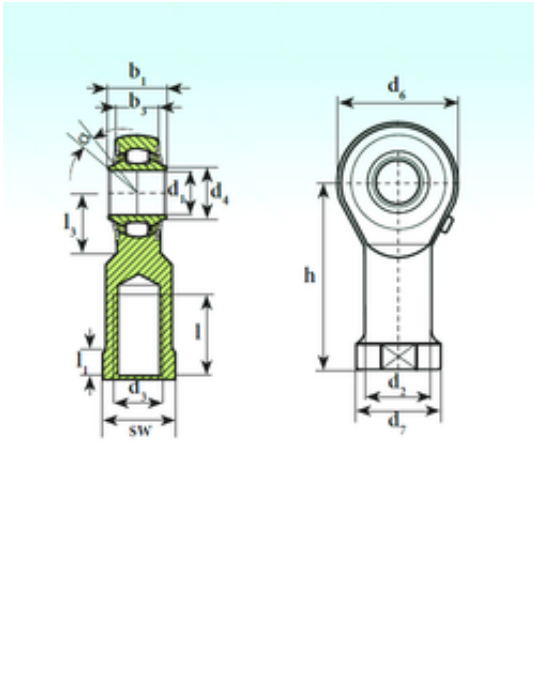
TSF 16 RB Bearing 2D drawings and 3D CAD models
